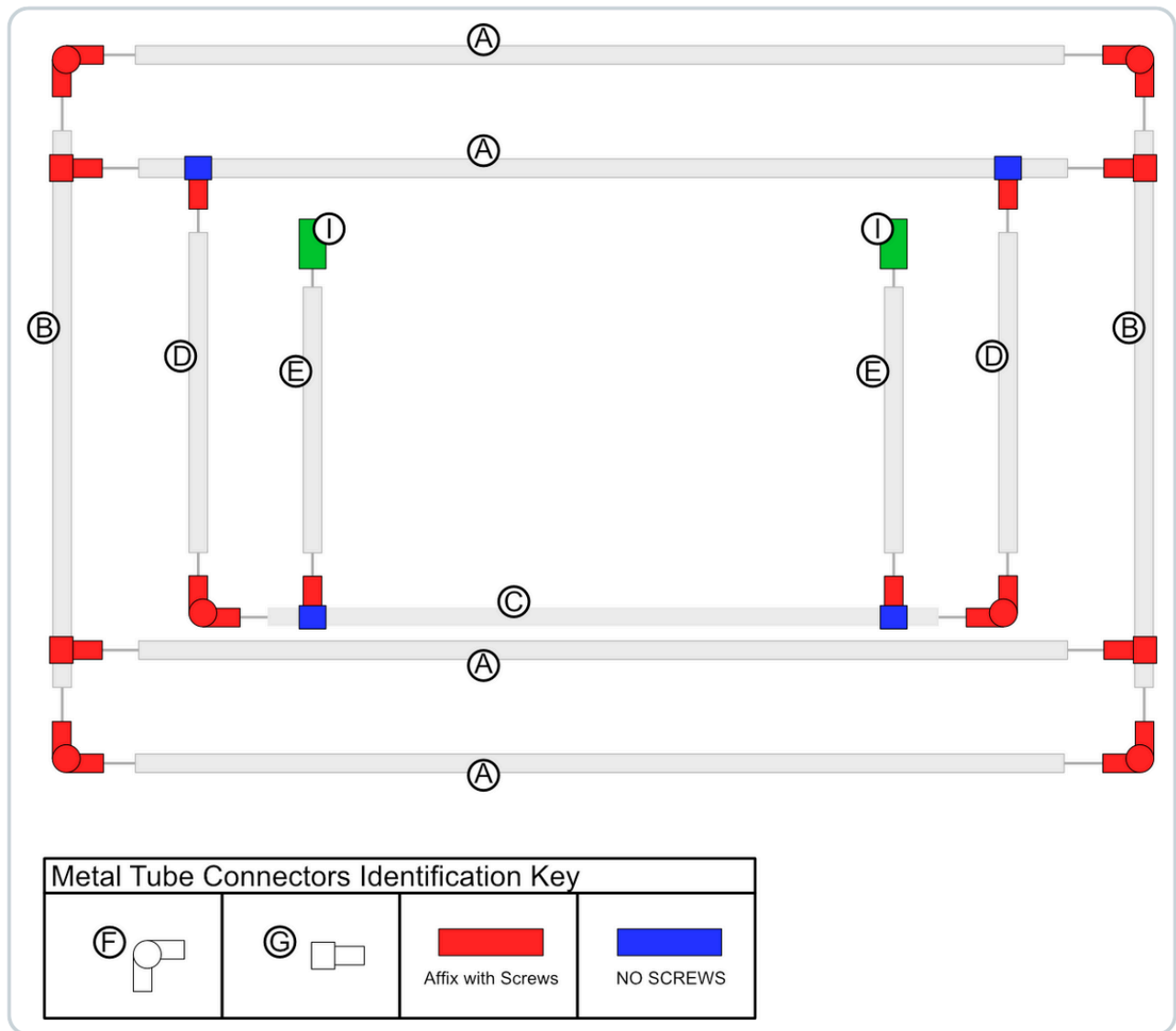
Figure 6: Exploded folded-state component and connector-fastening map.
