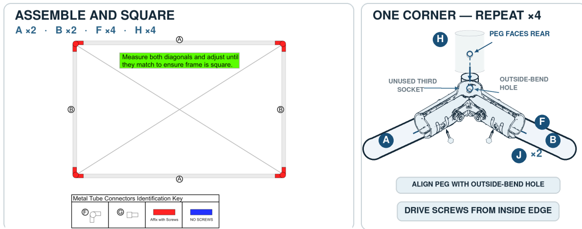
Figure 7: Stage 1 main-frame assembly and corner bracket detail.
