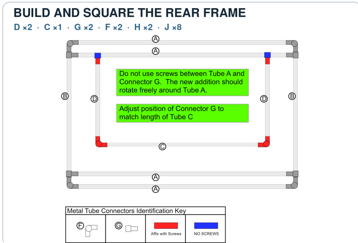
Figure 9: Stage 3 rear-support-frame assembly and hinge fastening.
