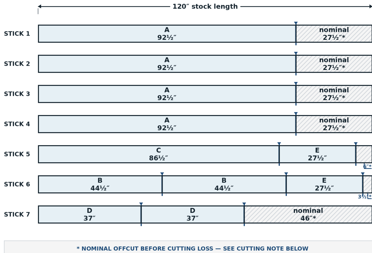
Figure 4: Proportional seven-stick conduit cut diagram.
