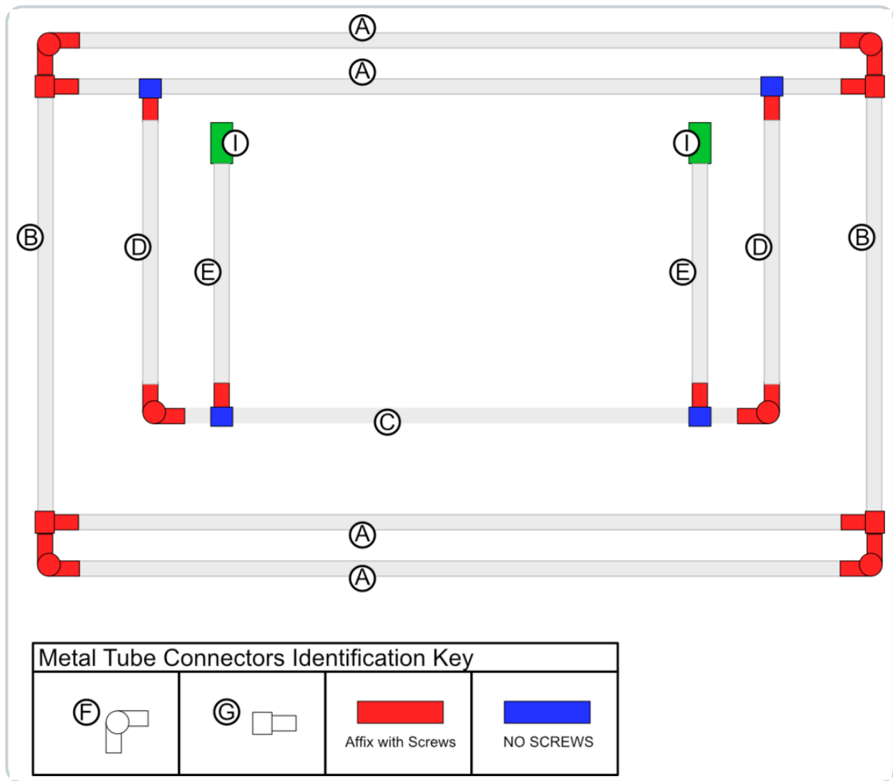
Figure 5: Folded-state component and connector-fastening map for the finished frame.
