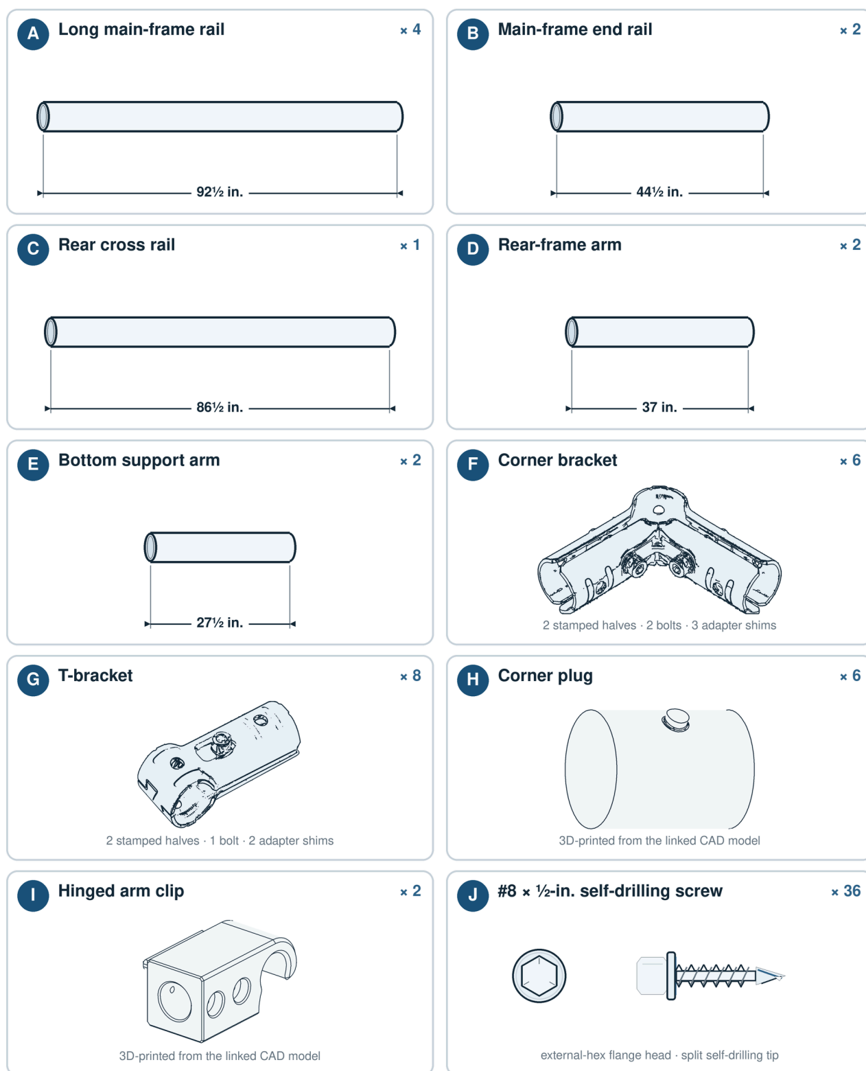
Figure 3: Component inventory for one complete sideline screen frame.
