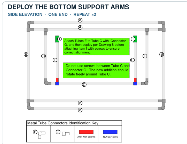
Figure 10: Stage 4 bottom support arm and clip installation.
