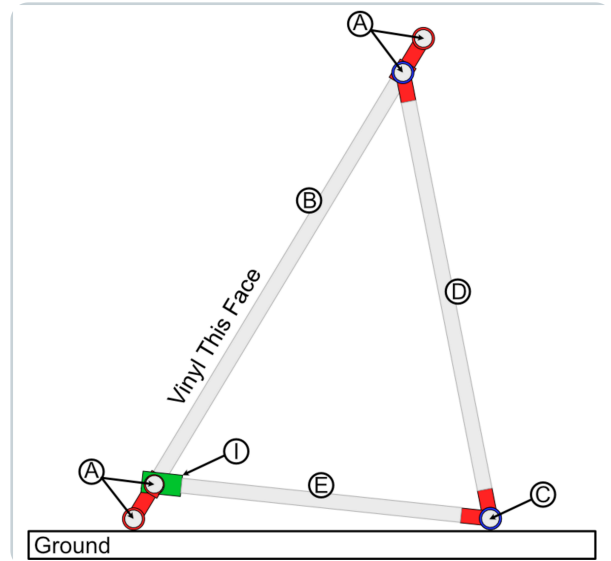
Figure 11: Deployed cutaway side elevation.
